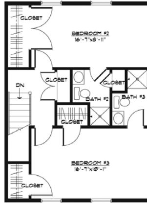
Upper Level
