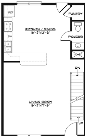
Entry Level
