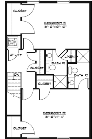
Upper Level
