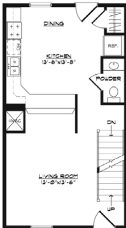
Entry Level
