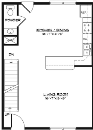
Entry Level
